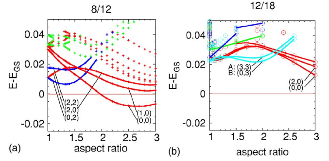
FIG. 11. (Color online) Energies of the half-polarized state under varying aspect ratio (Coulomb interaction, \frac{2}{3} ). (a) N=8 and (b) N=12 .
