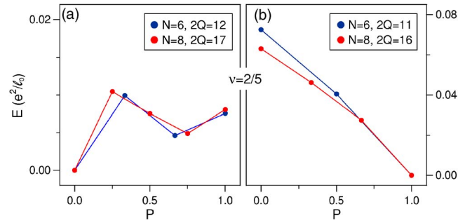
FIG. 1. (Color online) Excitation energy E as a function of electron spin polarization P , calculated on a sphere for N=6 and 8 electrons, at the values of 2Q corresponding to incompressible \nu=2/5 Jain states at P=0 (a) or P=1 (b).
