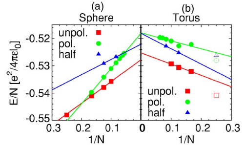
FIG. 4. (Color online) Energy per particle of the singlet state, half-polarized state (half-polarized state), and the fully polarized state at \nu=\frac{2}{3} . Different system sizes are shown ( N=4-18 electrons), extrapolation to infinite systems, 1/N \rightarrow 0 (only solid points were used).
