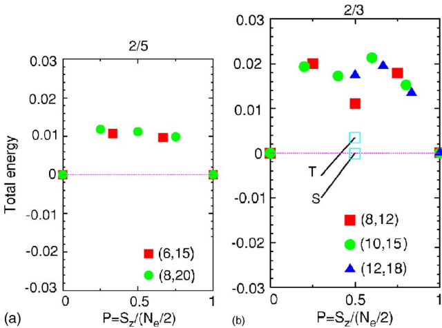
FIG. 3. (Color online) E(P) of the \frac{2}{5} and \frac{2}{3} systems on a torus. Here, the singlet and polarized states occur in systems with the same (N, N_m) , so that the E(P) dependence shown here is relevant in the whole range of P . The 1/N \rightarrow 0 extrapolated values are displayed by S (sphere) and T (torus).
