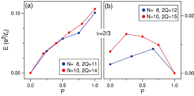
FIG. 2. (Color online) Same as Fig. 1, but \nu=2/3 and N=8, 10 .
