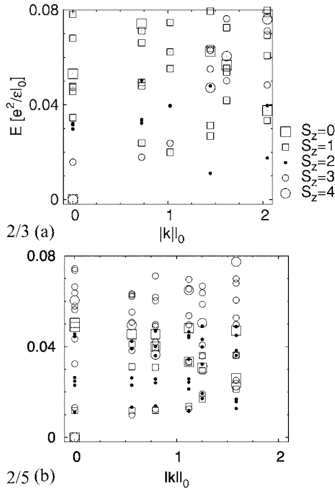
FIG. 8. Full spectrum of eight electrons at \nu=2/3 and 2/5 (hence both \nu^*=2 ) on a torus with Zeeman energy adjusted so that the fully polarized and spin-singlet incompressible states are degenerate. To be compared with \nu=2 , Fig. 7(b).
