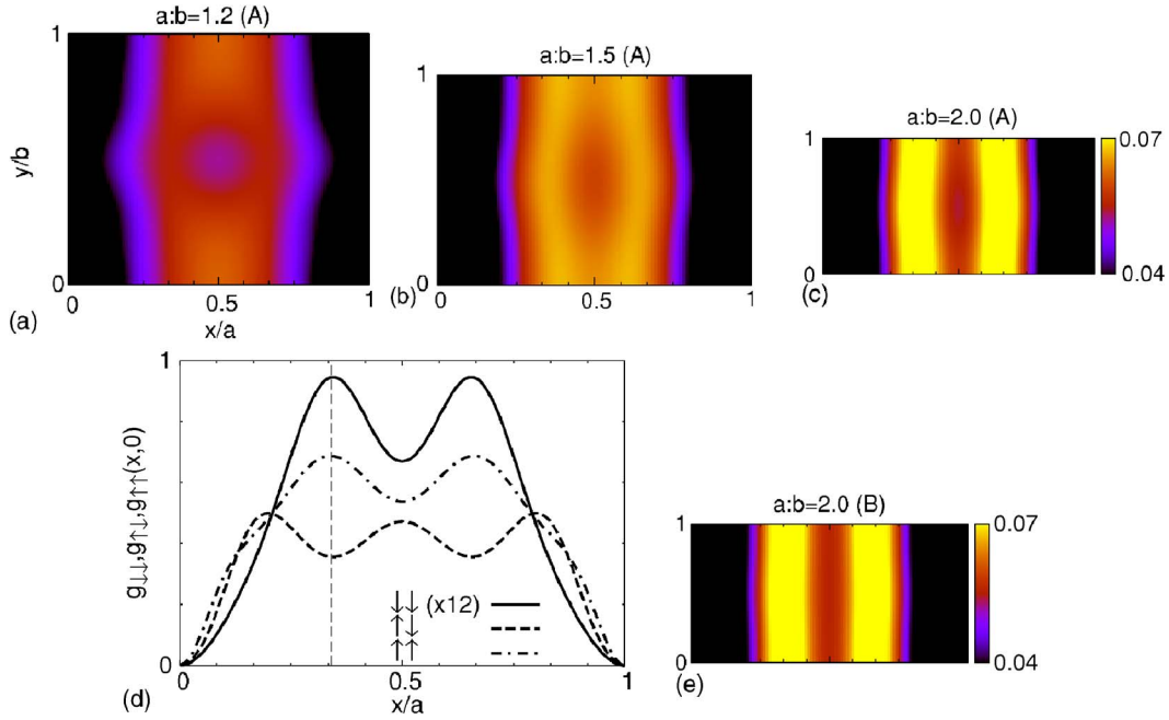
FIG. 12. (Color online) Correlation functions g(\vec{r})=g(x,y) of the \vec{k}_r/k_u=(3,3) half-polarized state [A in Fig. 11(b)]. Under slight variation of the aspect ratio \alpha=a:b , the conditional probability g_{\uparrow\uparrow}(\vec{r}) indicates antiferromagnetic ordering (a),(b),(c), confirmed by g_{\downarrow\downarrow} and g_{\uparrow\downarrow} (d). The state B from Fig. 11(b) has a very similar structure (e).
