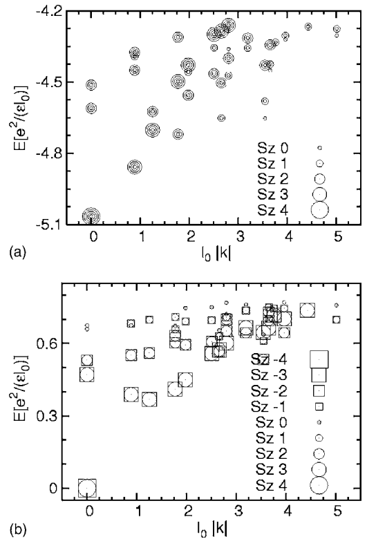
FIG. 7. Spectra of (a) \nu=1 and (b) \nu=2 quantum Hall ferromagnets. Eight electrons on a torus. The complete degeneracy of S_z = -S, -S+1, \dots, S levels (a) corresponds to a Heisenberg ferromagnet; the degeneracy of S_z and -S_z only (b) is proper to an Ising ferromagnet.
