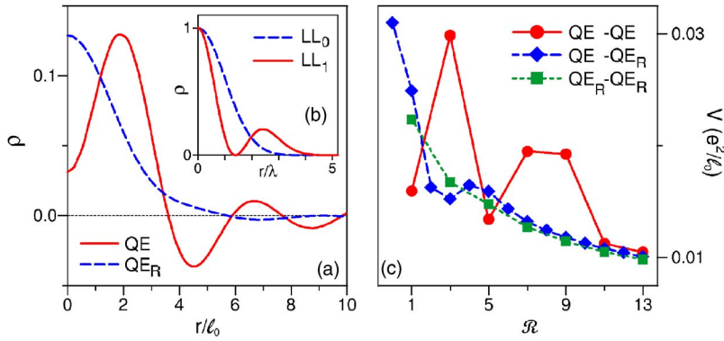
FIG. 5. (Color online) (a) Radial charge distributions of QE_R and QE at \nu=1/3 —i.e., of the CF's in the lowest and first excited LL. (b) Same for the electrons. (c) CF-CF interaction pseudopotentials at \nu=1/3 .
